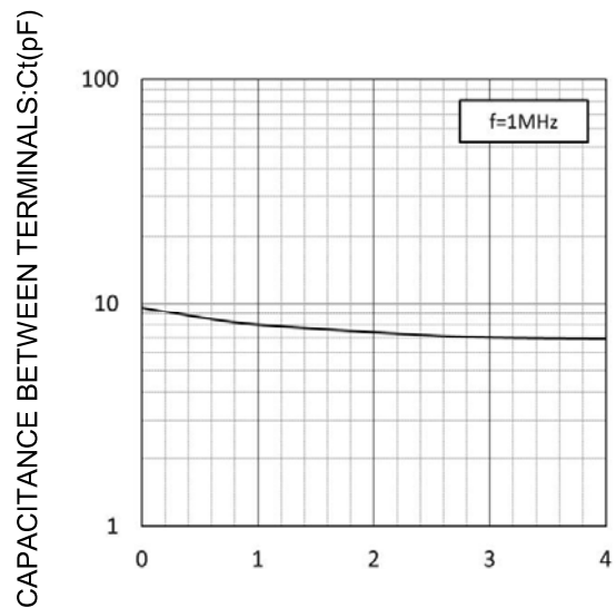
REVERSE VOLTAGE:VR(V) V_R - C_t CHARACTERISTICS
