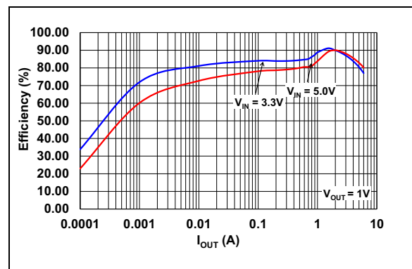
FIGURE 2-6: Efficiency vs. Load Current.
