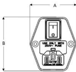
Class II, IEC 60320 C18
