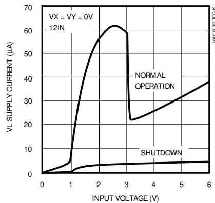
VL SUPPLY CURRENT vs. VL INPUT VOLTAGE
