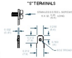
FITS PANELS UP TO 0.50in [12.7mm] THICK
