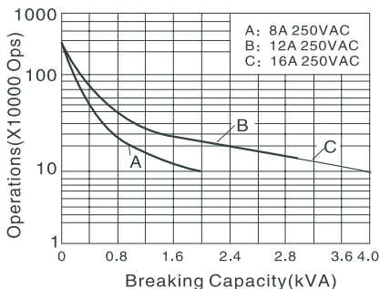
Endurance Curve
