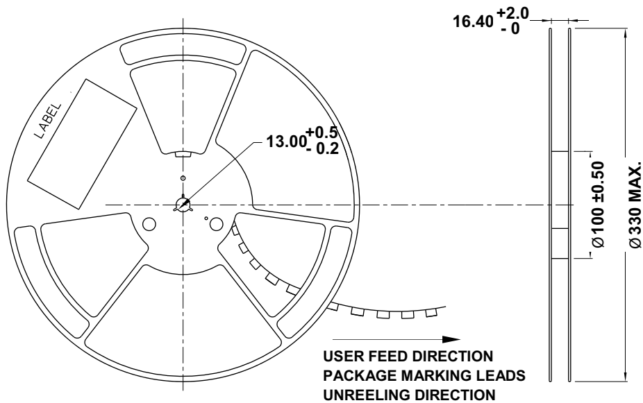
Figure 12: Reel Dimensions
