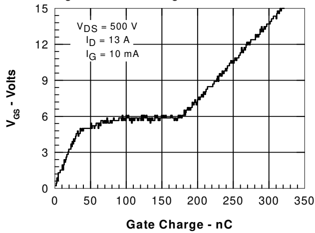
Figure 7. Gate Charge
