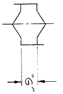
ENLARGED VIEW OF INSULATION CRIMP
