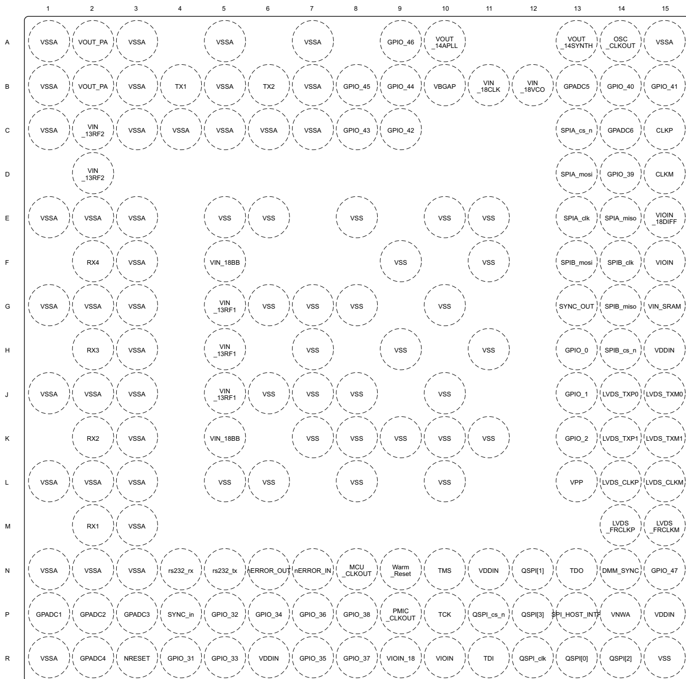
Figure 4-1. Pin Diagram
