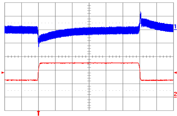
Fig. 5.0V.11: Output voltage response to load current step-change (2.5A – 5A – 2.5A) at Vin = 24V. Top trace: output voltage (100 mV/div.). Bottom trace: load current (2 A/div.). Current slew rate: 0.1 A/µs. Co = 1 µF ceramic. Time scale: 0.2 ms/div.
