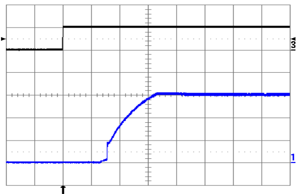
Fig. 1.5V.10: Turn-on transient at full rated load current (resistive) plus 10,000 µF at V in = 24V, triggered via ON/OFF pin. Top trace: ON/OFF signal (5 V/div.). Bottom trace: output voltage (0.5 V/div.). Time scale: 1 ms/div.
