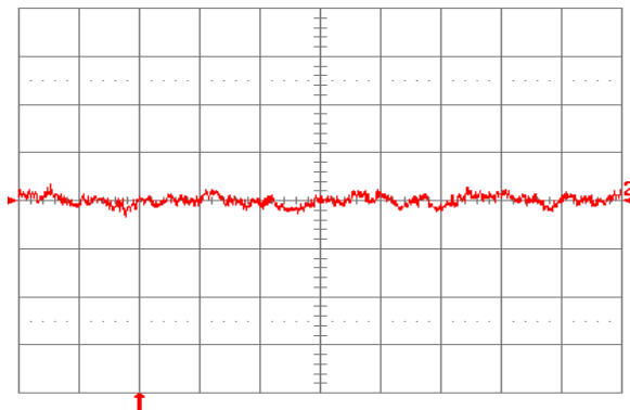
Fig. 2.0V.16: Input reflected ripple current, i_s (10 mA/div.), measured through 10 \mu\text{H} at the source at full rated load current and V_{in} = 24\text{V} . Refer to Fig. 2.0V.14 for test setup. Time scale: 1 \mu\text{s}/\text{div} .
