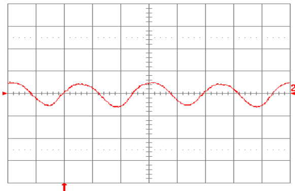
Fig. 2.0V.15: Input reflected ripple current, i_c (100 mA/div.), measured at input terminals at full rated load current and V_{in} = 24\text{V} . Refer to Fig. 2.0V.14 for test setup. Time scale: 1 \mu\text{s}/\text{div} .
