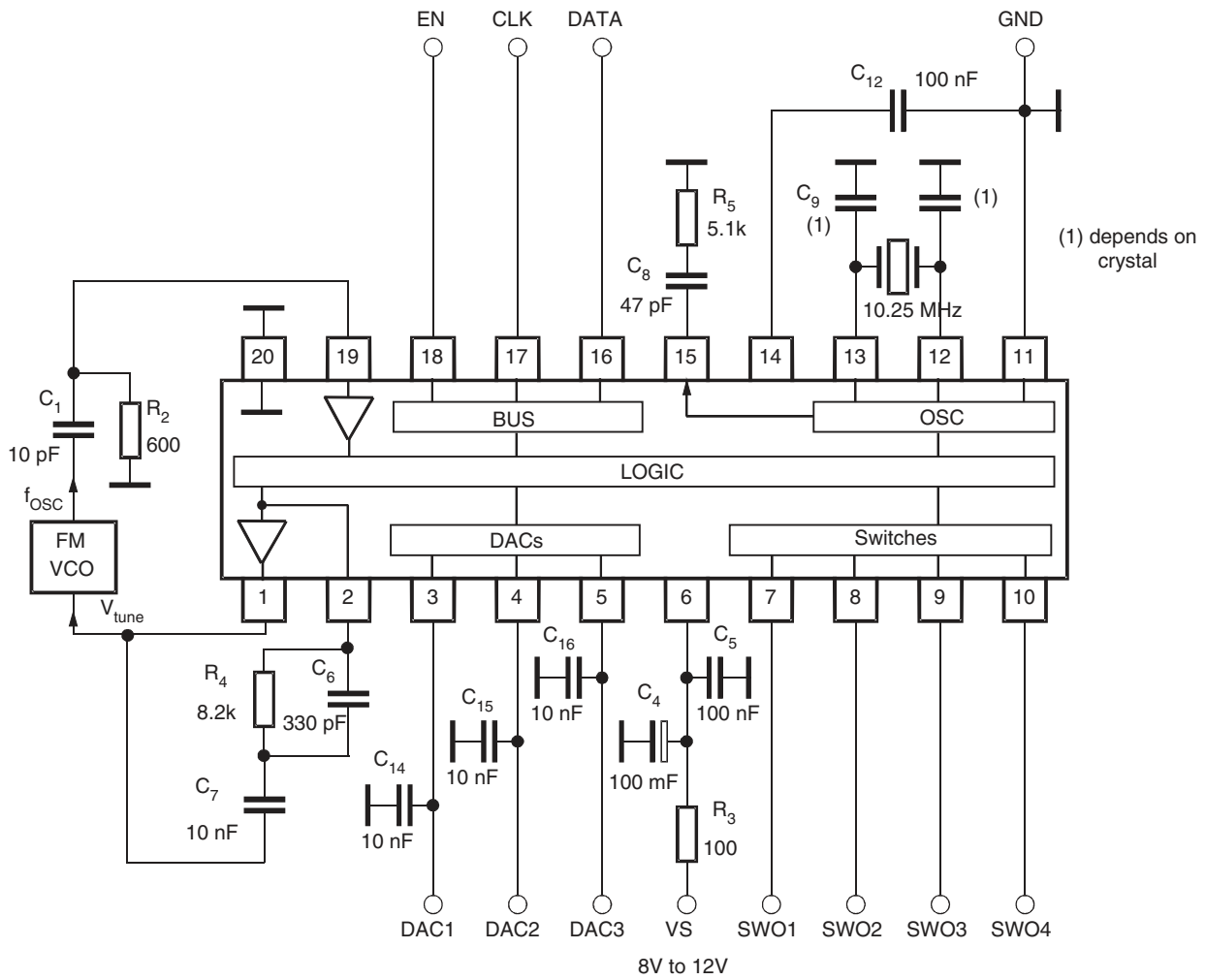
Figure 10-1. Application Circuit
