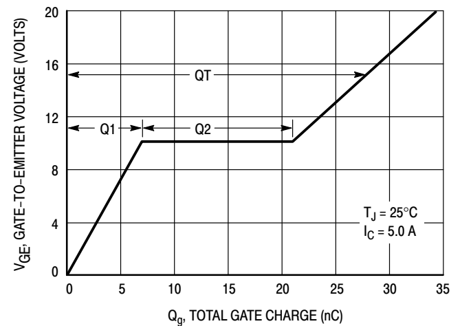
Figure 6. V_{GE} versus Total Charge
