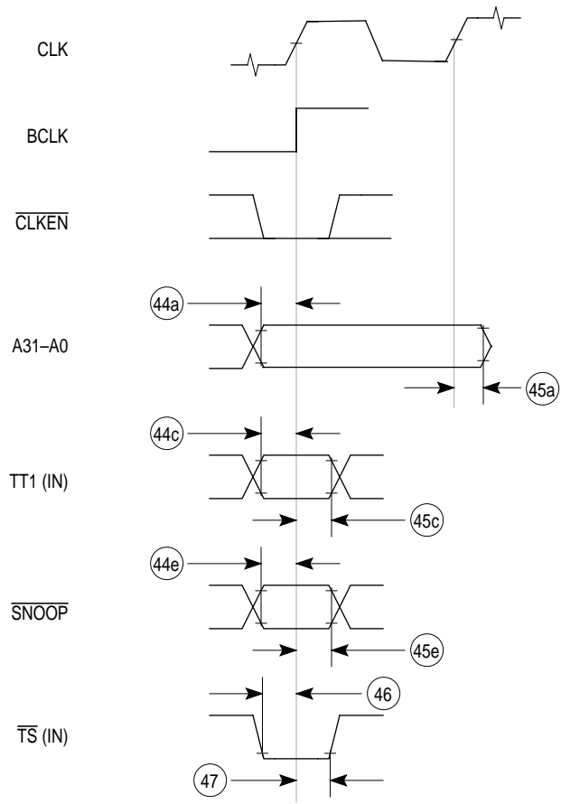
Figure 12-8. Snoop Timing
