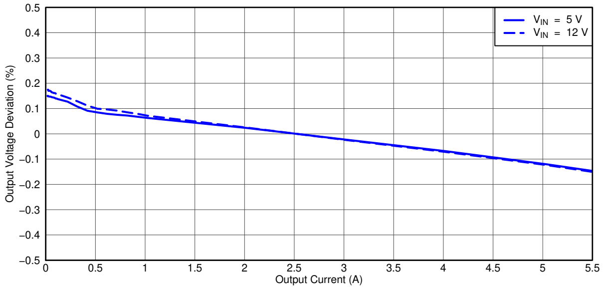
Figure 4-3. TPS54525EVM-608 Load Regulation
