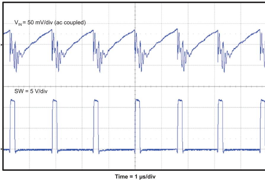
Figure 4-7. TPS54525EVM-608 Input Voltage Ripple
