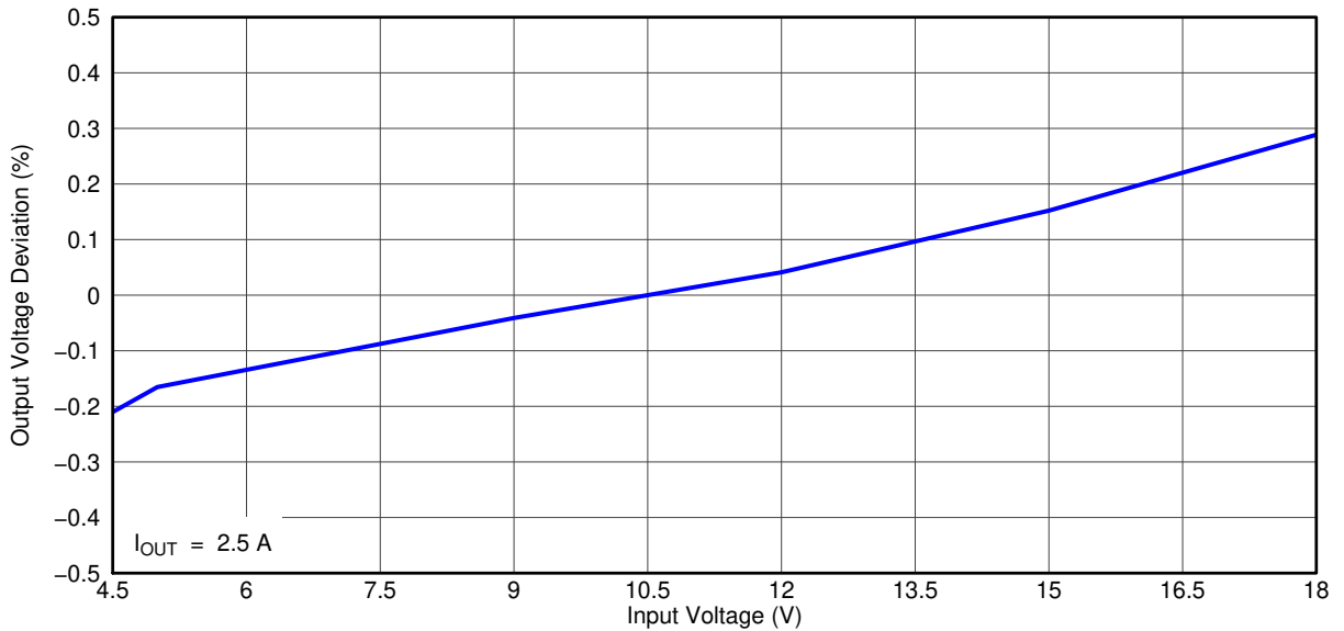
Figure 4-4. TPS54525EVM-608 Line Regulation
