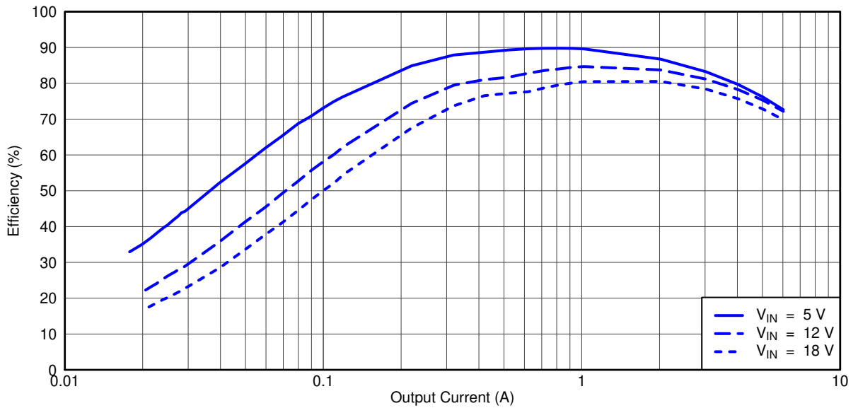
Figure 4-2. TPS54525EVM-608 Light Load Efficiency
