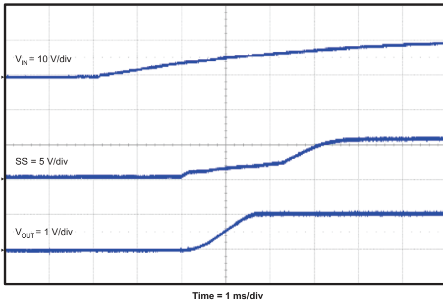
Figure 4-8. TPS54525EVM-608 Start-Up Relative to V_{IN}
