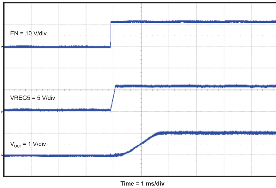
Figure 4-9. TPS54525EVM-608 Start-Up Relative to EN
