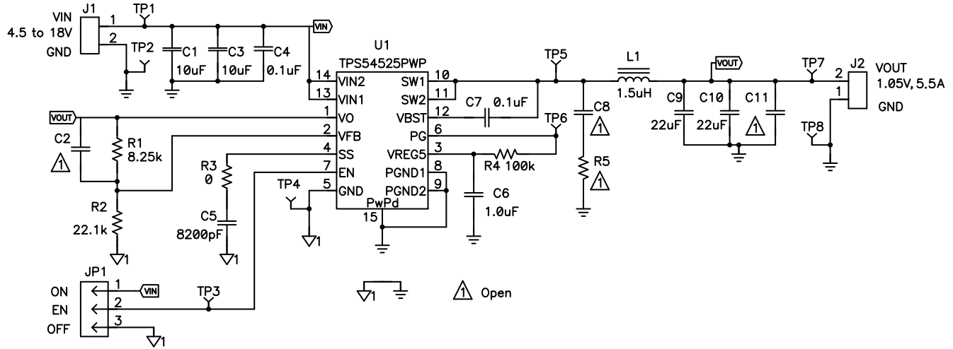
Figure 6-1. TPS54525EVM-608 Schematic Diagram
