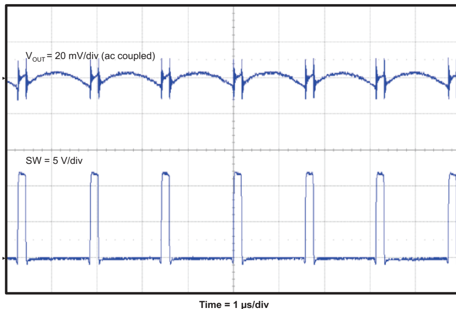
Figure 4-6. TPS54525EVM-608 Output Voltage Ripple
