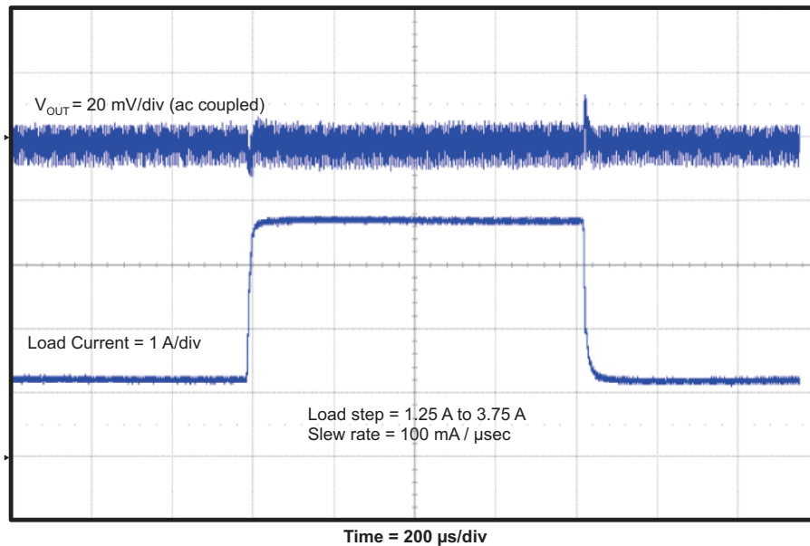
Figure 4-5. TPS54525EVM-608 Load Transient Response
