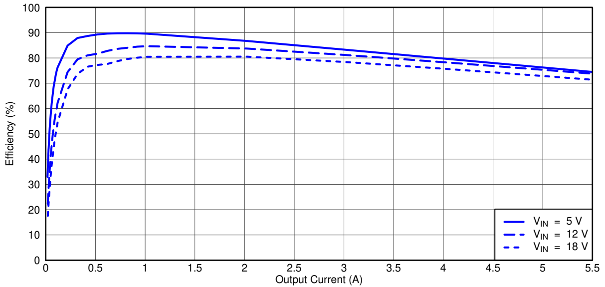
Figure 4-1. TPS54525EVM-608 Efficiency
