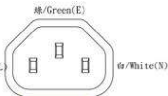
插頭端面圖 (Dimensions of Plug Face)
