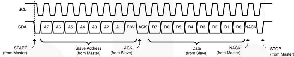
Figure 5. I²C Read
