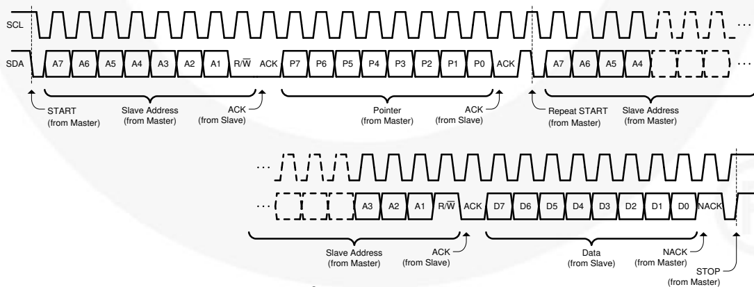
Figure 8. I²C Write Followed by Read
