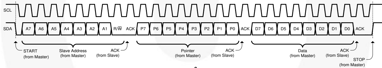
Figure 7. I²C Write
