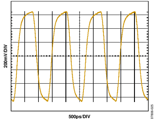
Figure 14. Typical Output Waveform, LVPECL (805 MHz)
