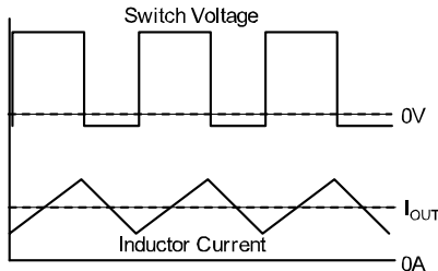
Figure 2. Continuous Operation
