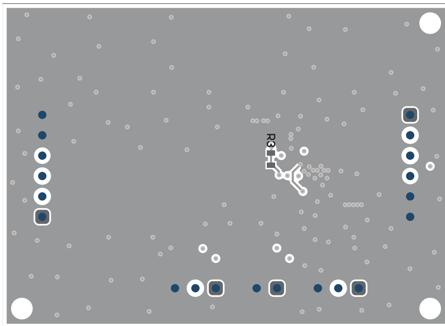
Figure 5-6. Bottom Assembly
