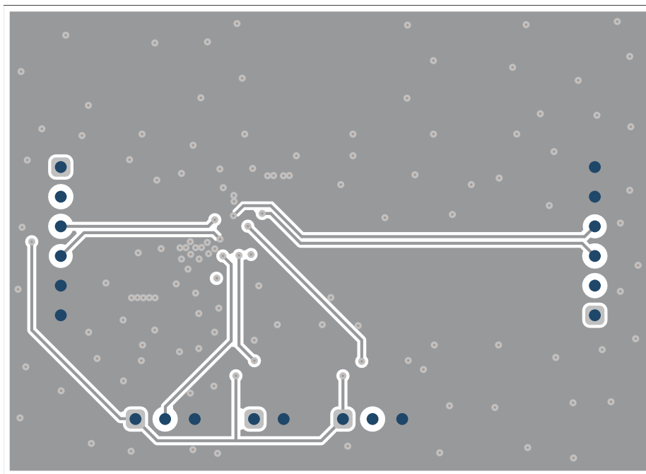
Figure 5-4. Signal Layer 2
