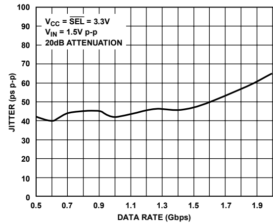
Figure 20. Jitter vs. Data Rate; PRBS 31
