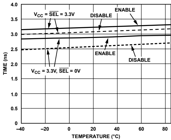
Figure 18. Enable/Disable Time vs. Temperature
