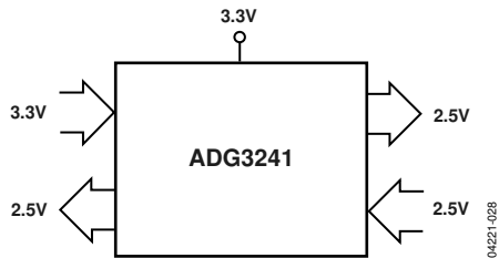
Figure 28. 3.3 V to 2.5 V Voltage Translation, \overline{SEL} = V_{CC}
