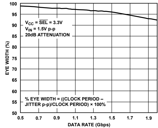
Figure 21. Eye Width vs. Data Rate; PRBS 31
