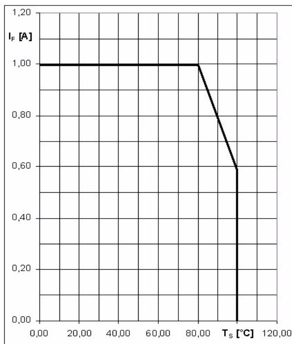
Maximal zulässiger Durchlassstrom Max. Permissible Forward Current I_F = f(T_S) ; for blue chip operated
