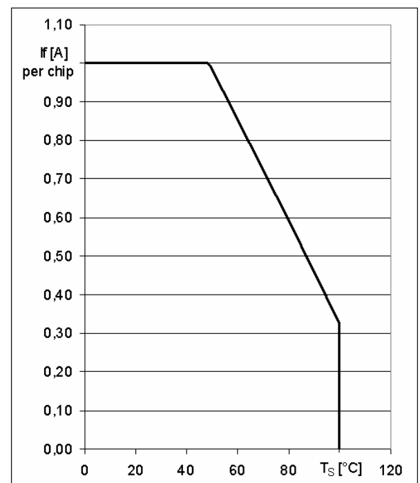
Maximal zulässiger Durchlassstrom Max. Permissible Forward Current I_F = f(T_S) ; for 4 chips operated
