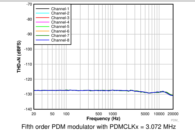
Figure 6. THD+N vs Input Frequency With a -20-dBr Input
