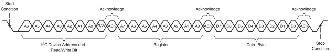
Figure 80. I 2 C Single-Byte Write Transfer
