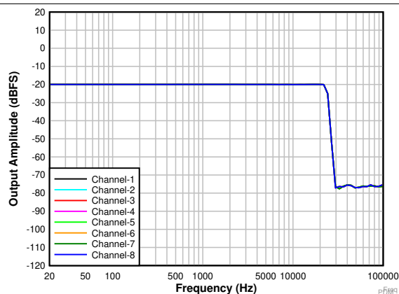
Fourth order PDM modulator with \text{PDMCLKx} = 1.536\text{ MHz}
