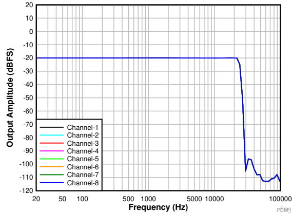
Fourth order PDM modulator with \text{PDMCLKx} = 3.072\text{ MHz}
