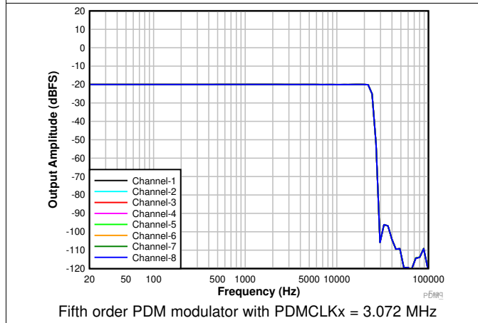
Figure 7. Frequency Response With a -20-dBr Input
