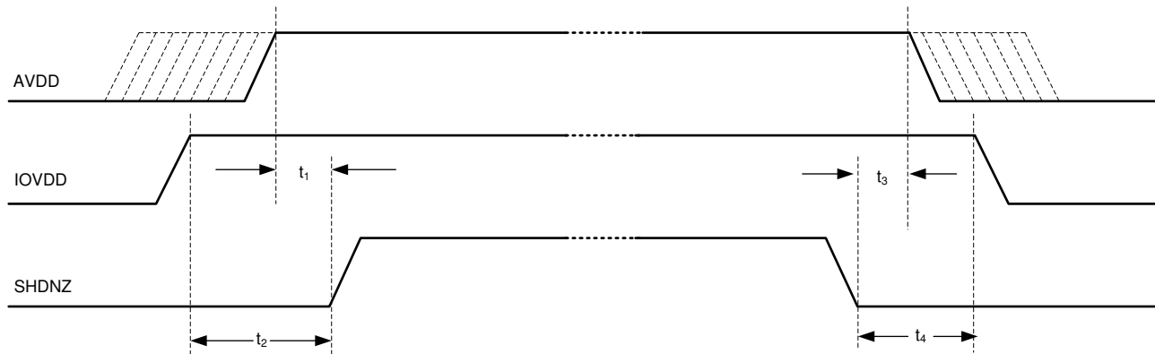
Figure 164. Power-Supply Sequencing Requirement Timing Diagram
