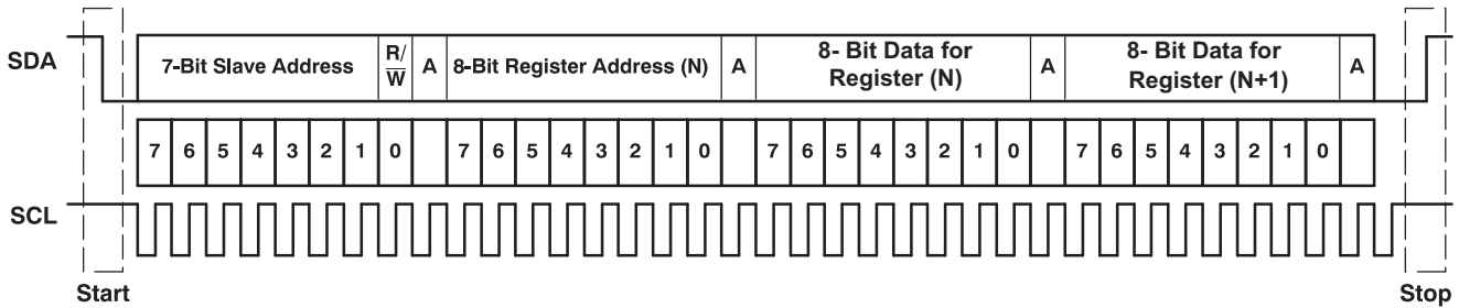
Figure 79. Typical I 2 C Sequence
