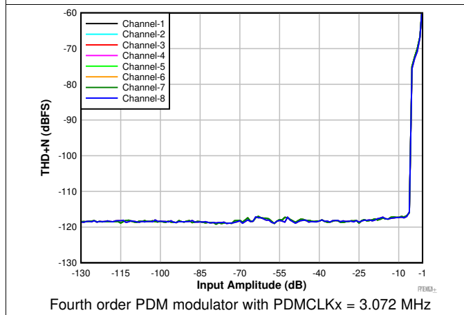
Figure 9. THD+N vs Input Amplitude
