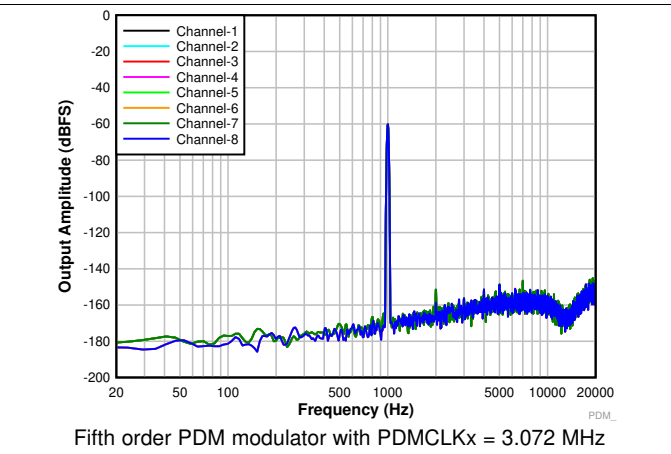
Figure 8. FFT With a -60-dBr Input
