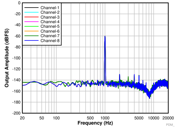
Fourth order PDM modulator with \text{PDMCLKx} = 3.072\text{ MHz}
