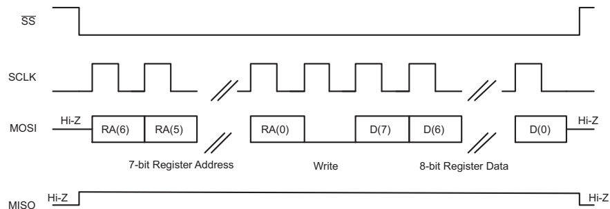
Figure 84. SPI Single-Byte Write Transfer
