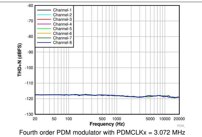
Figure 10. THD+N vs Input Frequency With a -20-dBr Input
