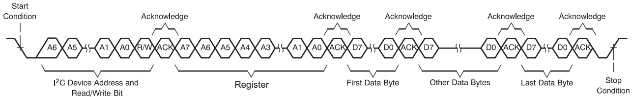
Figure 81. I 2 C Multiple-Byte Write Transfer
