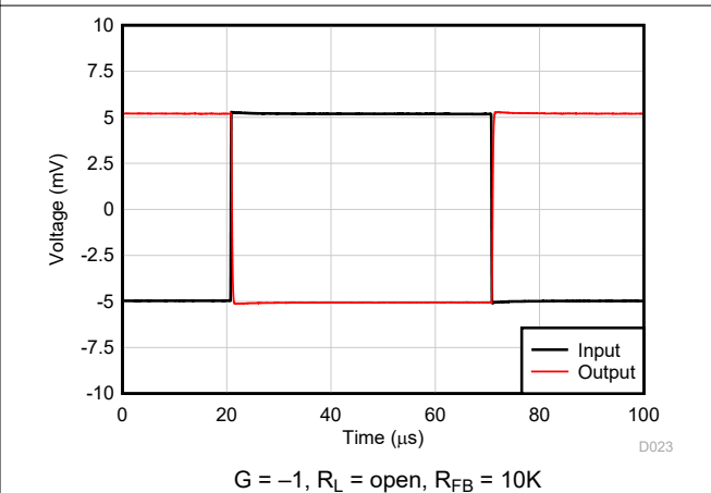
Figure 6-28. Overload Recovery
