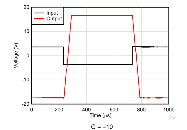
Figure 6-28. Overload Recovery
