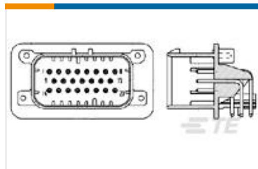
TE Part #770669-1 23POS,PIN DIA 1.3,HDR ASSY,90DEG, COD 1
