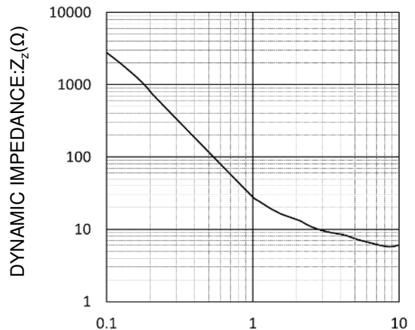
ZENER CURRENT: I_z (mA) I_z - Z_z CHARACTERISTICS
