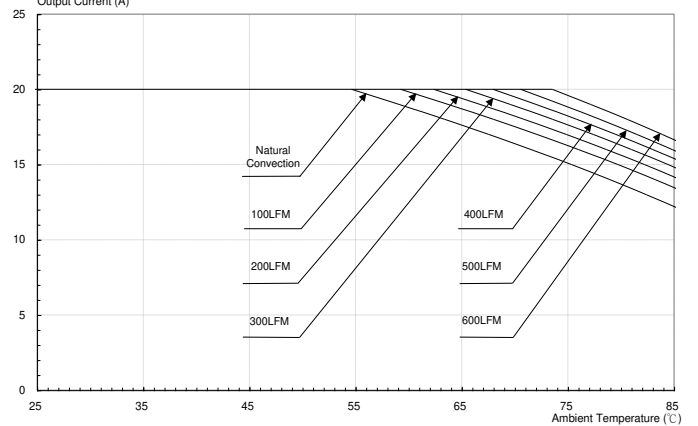
Figure 44: Output current vs. ambient temperature and air velocity @ Vin=12V, Vout=3.3V(Either Orientation)
