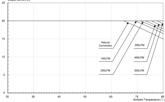
Figure 42: Output current vs. ambient temperature and air velocity @ Vin=12V, Vout=1.2V(Either Orientation)
