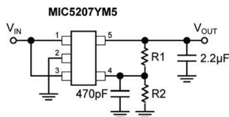
Figure 3. Ultra-Low-Noise Adjustable Voltage Application
