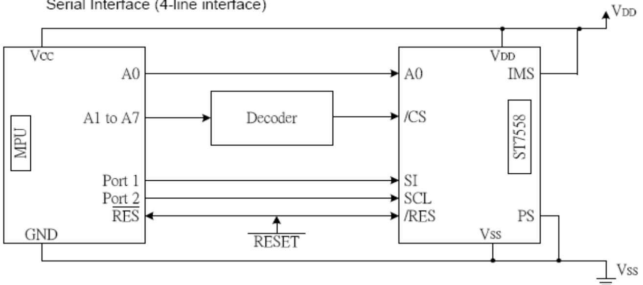
Serial Interface (4-line interface)
