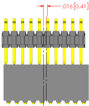
INITIAL X AXIS LINEAR MISALIGNMENT
