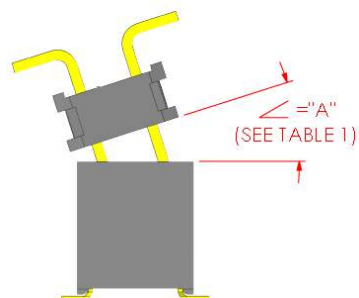
INITIAL X AXIS ANGULAR MISALIGNMENT
