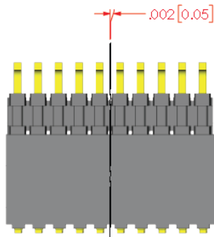
FINAL X AXIS LINEAR MISALIGNMENT
