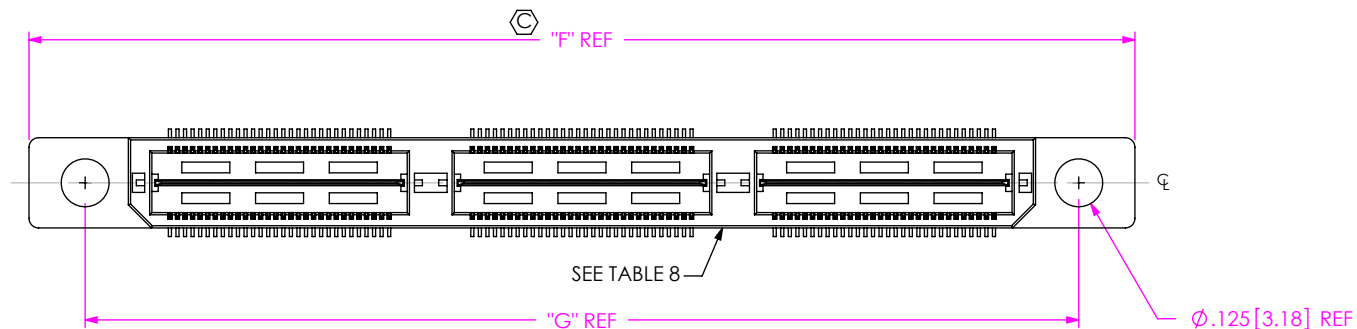
FIG 8 (QTH-090-01-X-D-GP SHOWN) (SAME AS FIG 1, EXCEPT AS SHOWN) (AVAILABLE ON -01 & -02 ONLY)
