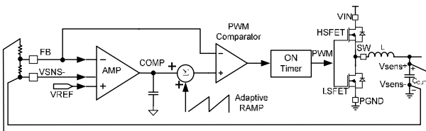
Figure 2: COT Control
