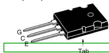
TO-264 (IXGK)
