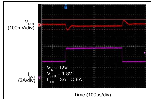
FIGURE 2-35: Transient Response, MIC45205-1 ( I_{OUT} = 3\text{A} to 6\text{A} ).
