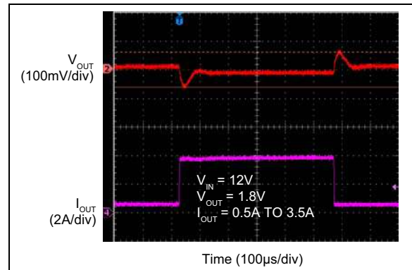
FIGURE 2-36: Transient Response, MIC45205-1 ( I_{OUT} = 0.5\text{A} to 3.5\text{A} ).
