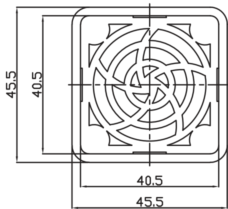
UPPER HOUSING
