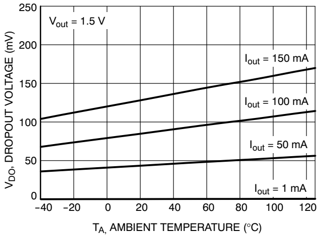
Figure 9. Dropout Voltage vs. Temperature (Over Current Range)
