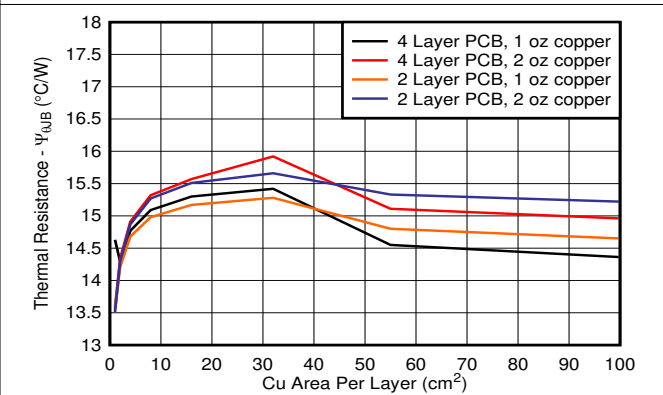
Figure 8-5. \psi_{JB} vs Copper Area 2s2p DCY Package
