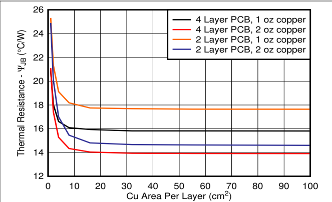
Figure 8-3. \psi_{JB} vs Copper Area 2s2p DRB Package
