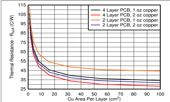
Figure 8-2. R_{\theta JA} vs Copper Area 2s2p DRB Package
