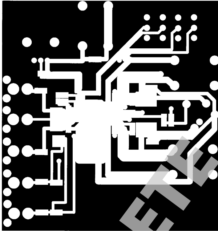
Layer 2 - ( Not to Scale )
