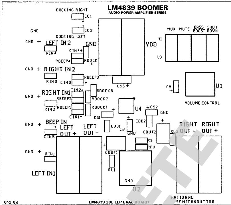
33X 34 LM4839 28L LLP EVAL BOARD NATIONAL SEMICONDUCTOR 20013478
