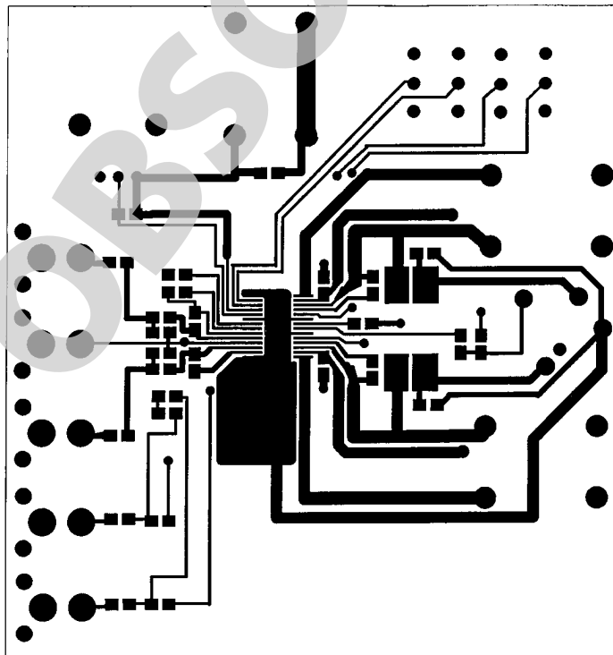
Top Layer - ( Not to Scale )
