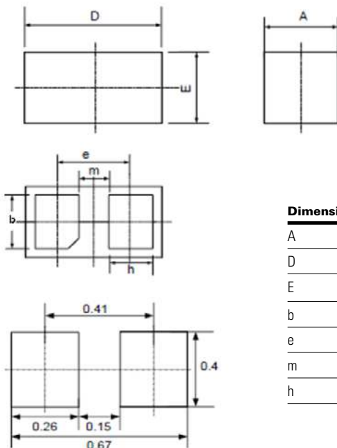
Land Pattern
