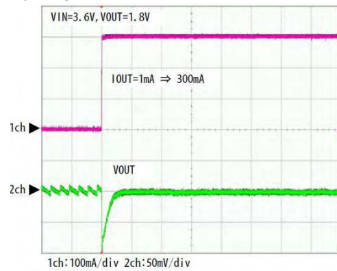
Ch1 – I_{OUT} , Ch2 – V_{OUT} 50 mV/div, Time – 200 \mu s/div
