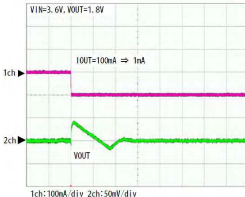
Ch1 – I OUT , Ch2 – V OUT 50 mV/div, Time – 200 µs/div
