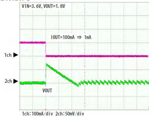
Ch1 – I_{OUT} , Ch2 – V_{OUT} 50 mV/div, Time – 200 \mu s/div
