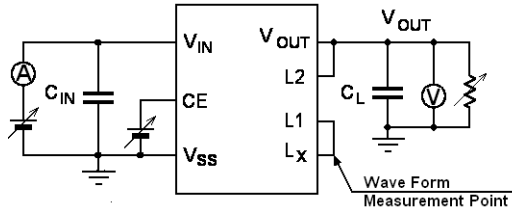
Circuit ①
