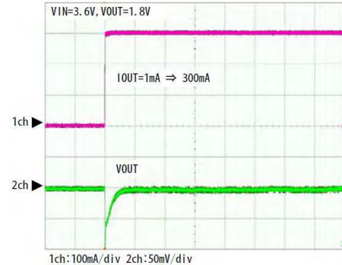
Ch1 – I OUT , Ch2 – V OUT 50 mV/div, Time – 200 µs/div
