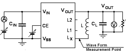
Circuit ⑧
