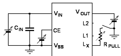
Circuit ⑥
