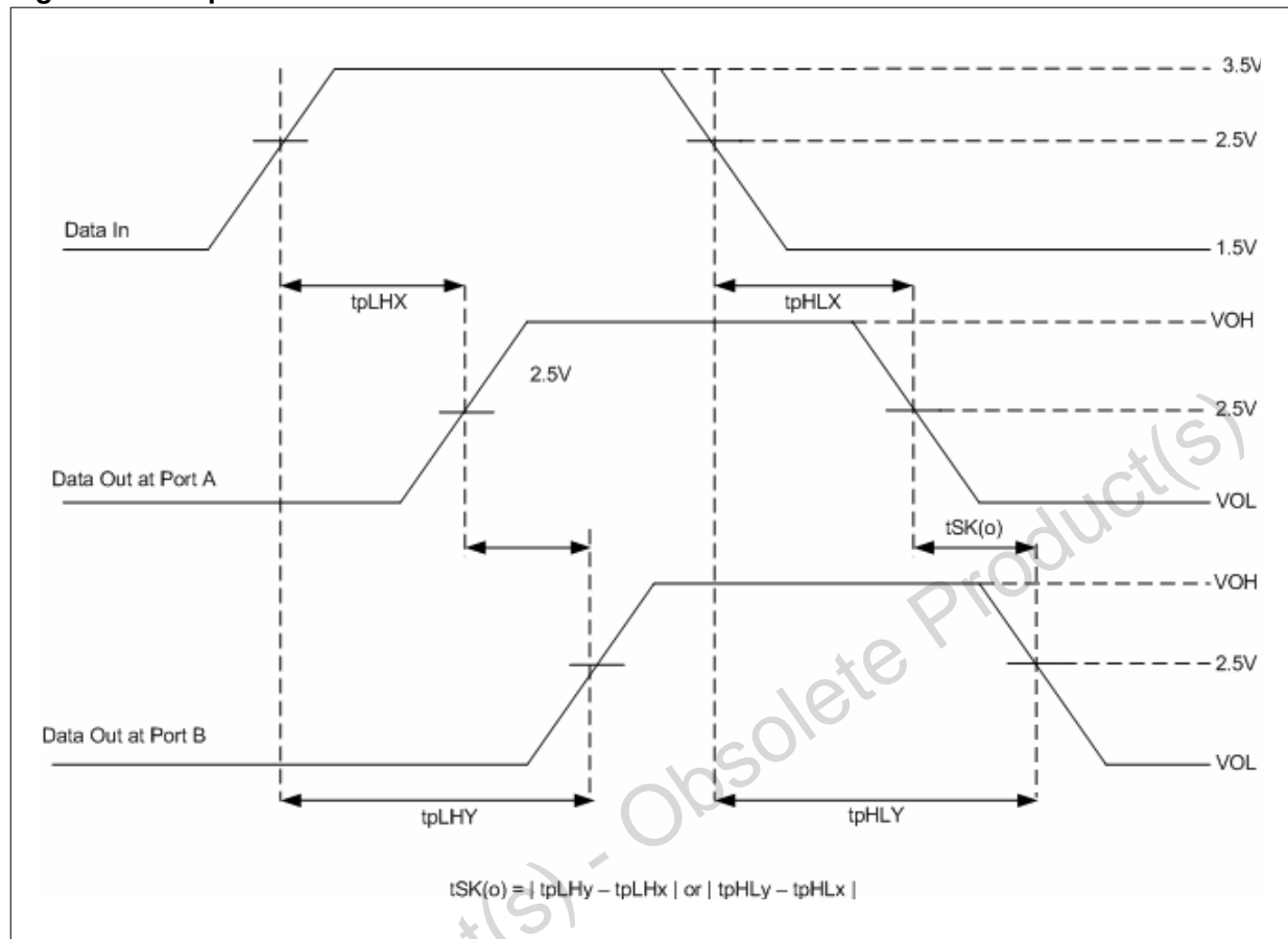
Figure 11. Pulse skew
