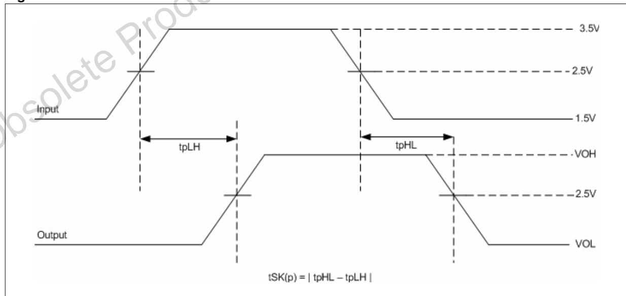
Figure 11. Pulse skew
