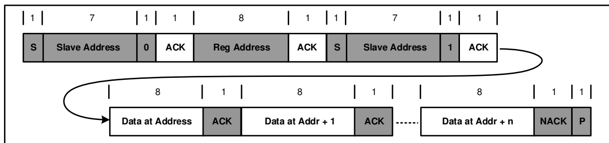
Figure 15: Multi-Read
