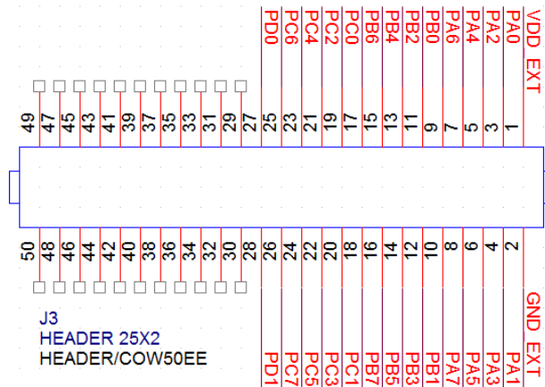
Fig.6: J3 schematic diagram
