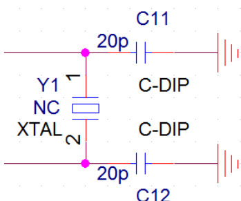
Fig.12: External Crystal & capacitor Y1, C11&C12
