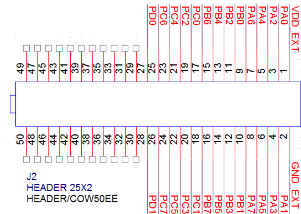
Fig.7: J2 schematic diagram
