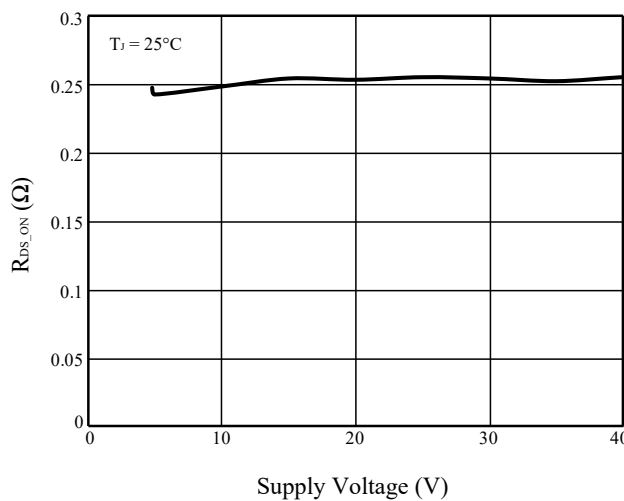
Figure 6 R_{DS\_ON} vs. V_{CC}
