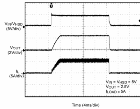
Power-Up/Power-Down Waveform
