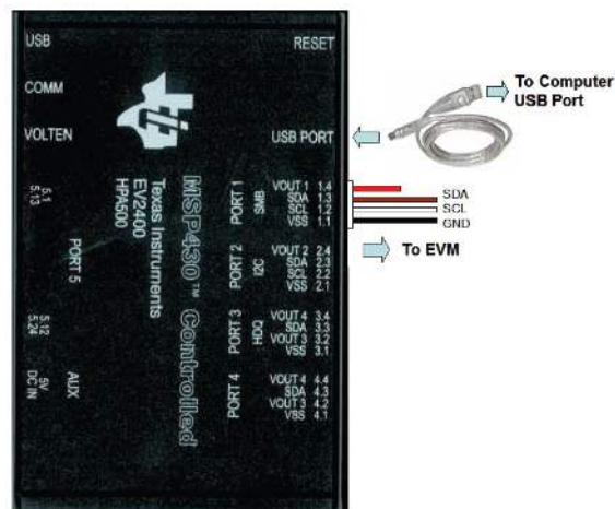
Figure 2-1. EV2400 Connections
