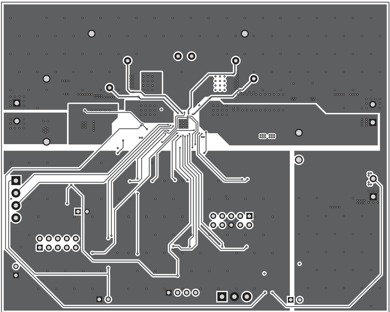
Figure 3-5. PCB Layer 3
