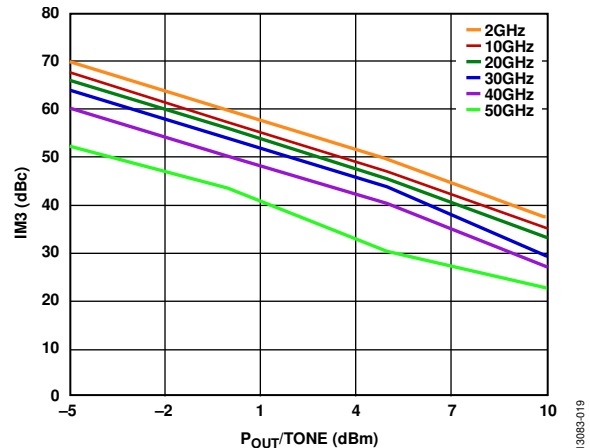
Figure 25. Output IM3 vs. P_{OUT}/Tone at V_{DD} = 4 V, V_{GG2} = 1.4 V
