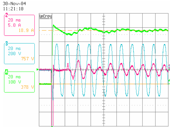
264VAC Startup @ 300W Load
