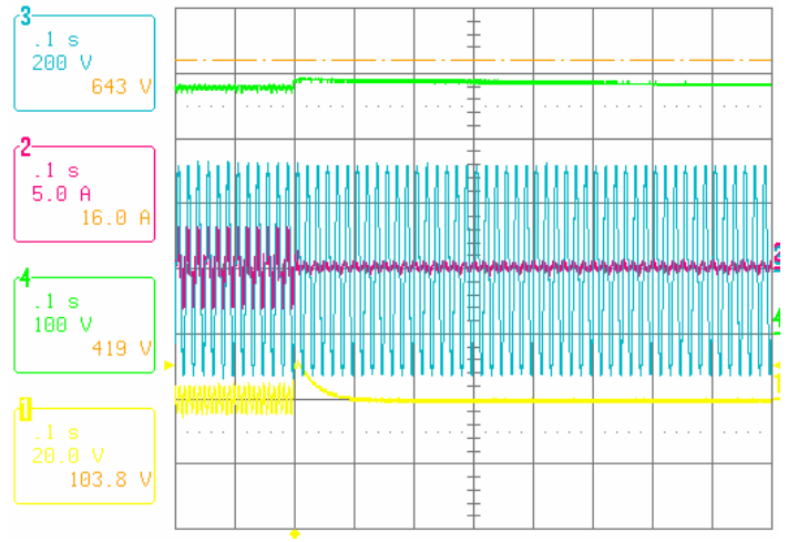
300W to No Load Step @ 230VAC
