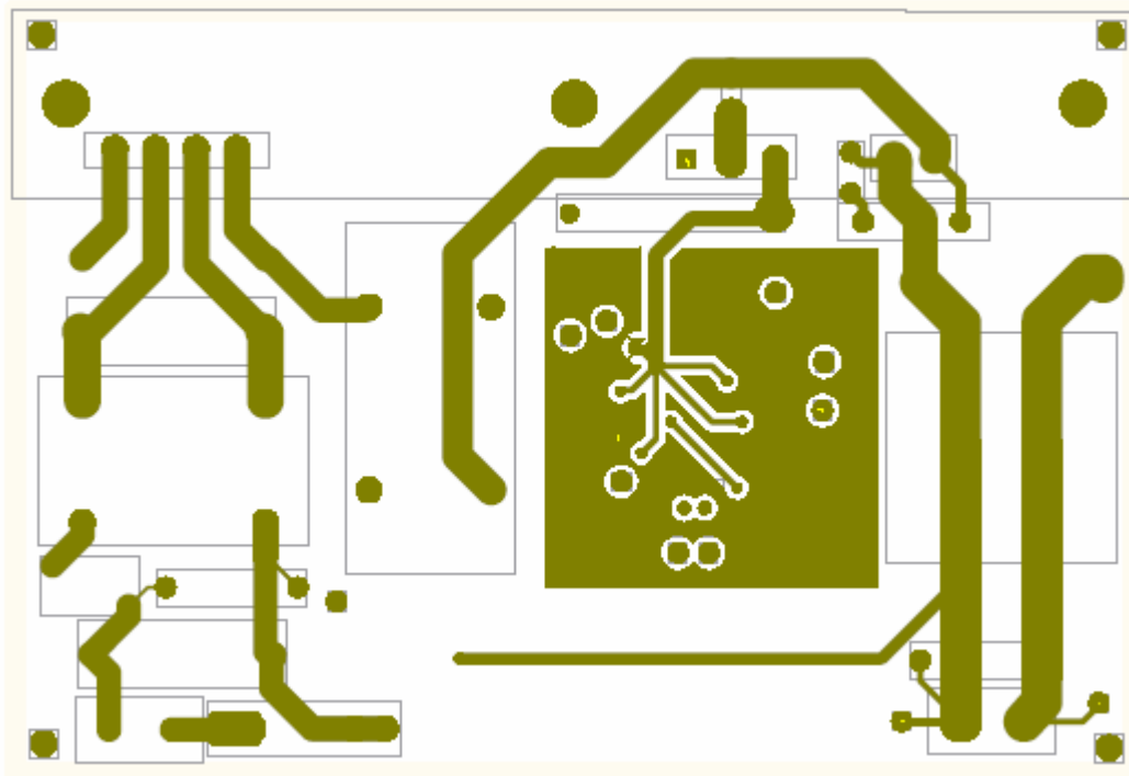
Figure 5 - Demo Board Bottom Layer Copper
