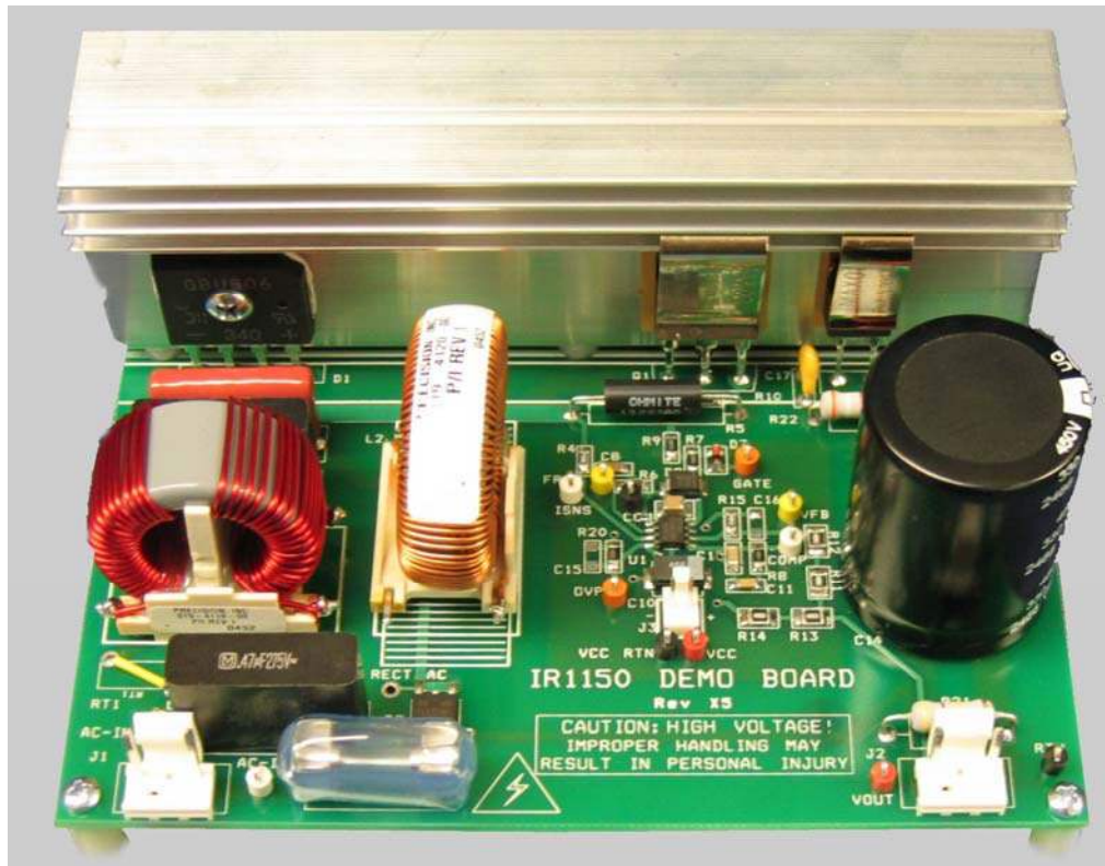
Figure 3 - Demo Board Photo
