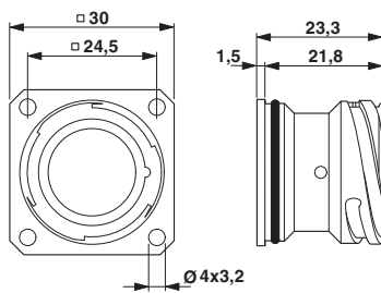
Dimensioned drawing
