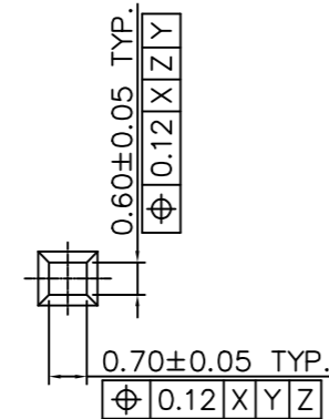
DETAIL II SCALE 4:1
